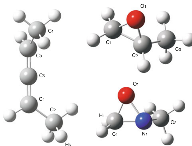
Fig. 1 ( R a )-1,3-dimethylallene, (2 R )-2-methyloxirane, and (2 R )- N -methyloxaziridine
